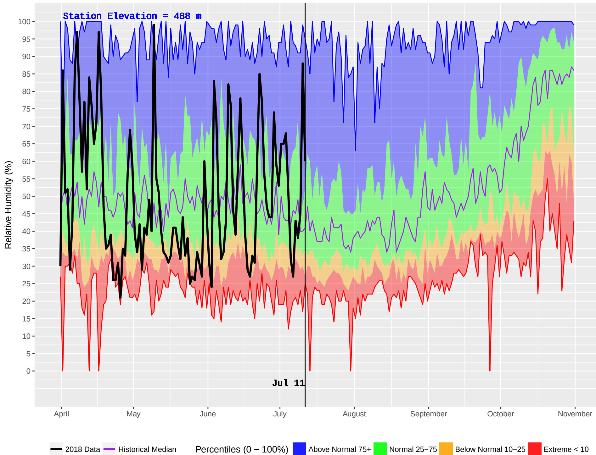
MABEL LAKE 2 (362) : Historical (1987–2016) and Current (2018) Noon Relative Humidity
