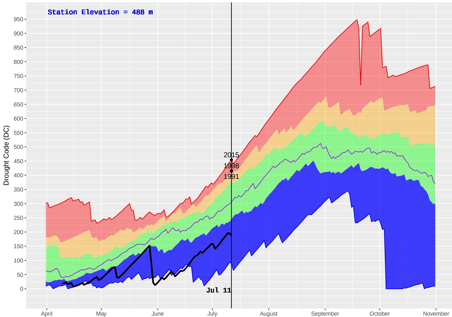
MABEL LAKE 2 (362) : Historical (1987–2016) and Current (2018) Noon Drought Code (DC)
